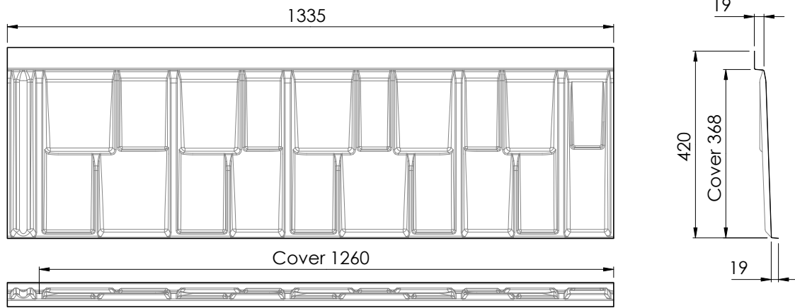
Figure 5.1 Tile Dimensions
