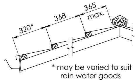
Figure 5.5 Batten Layout
