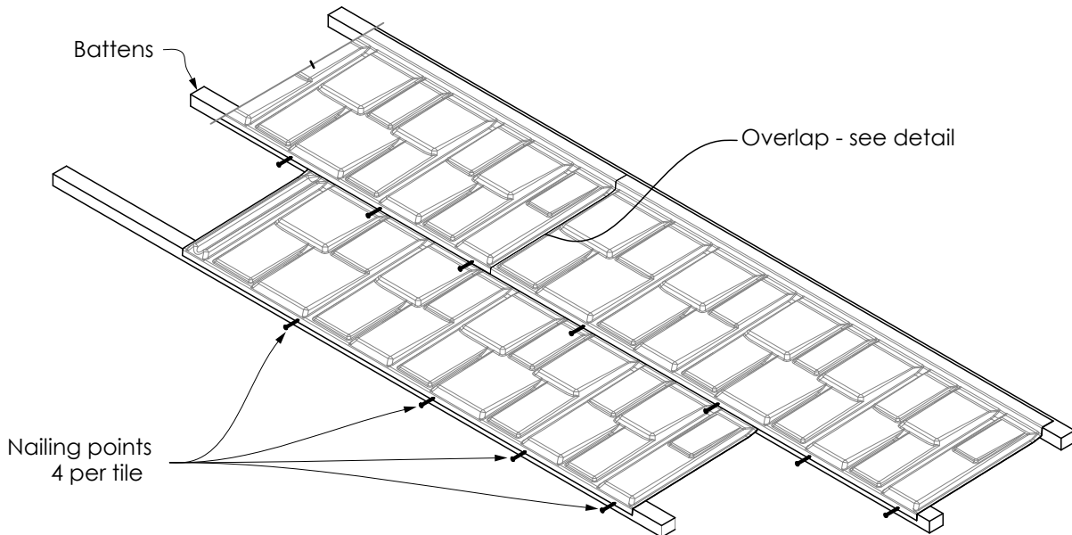
Figure 5.2 Nailing Detail
