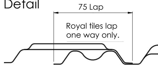
Figure 5.4 Lap Section
