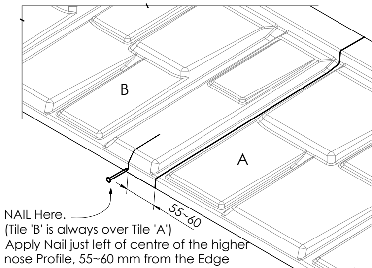
Figure 5.3 Overlap Detail
