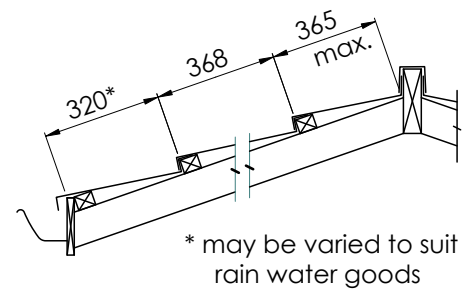
Figure 1.5 Batten Layout
