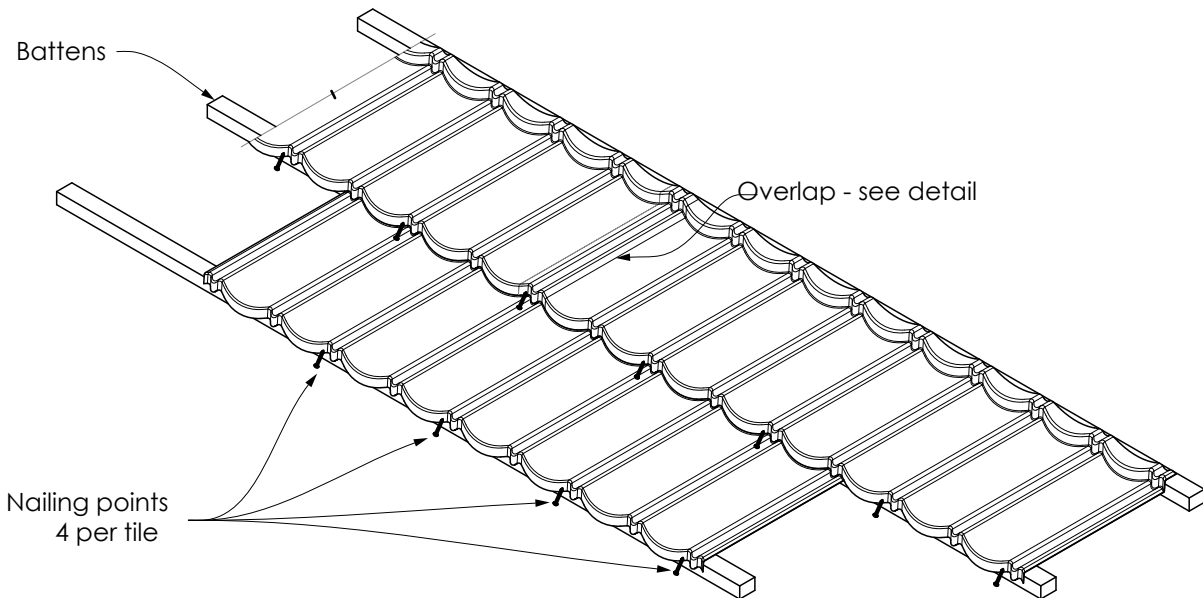
Figure 1.2 Nailing Detail
