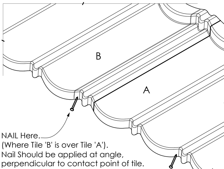
Figure 1.3 Overlap Detail
