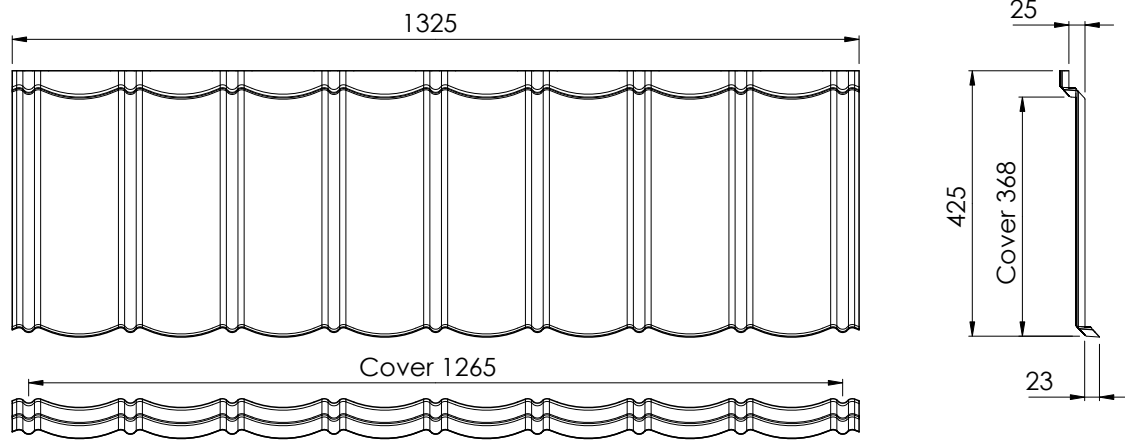
Figure 1.1 Tile Dimensions
